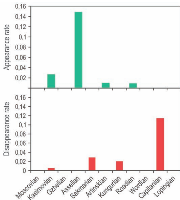
Figure 5. Per-capita rates of appearance and disappearance for spores and pollen grains.
