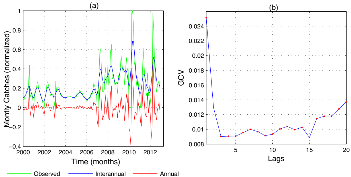
Figure 2. (a) Normalized shrimp catches, interannual and annual components (b) Lagged values calibration.
